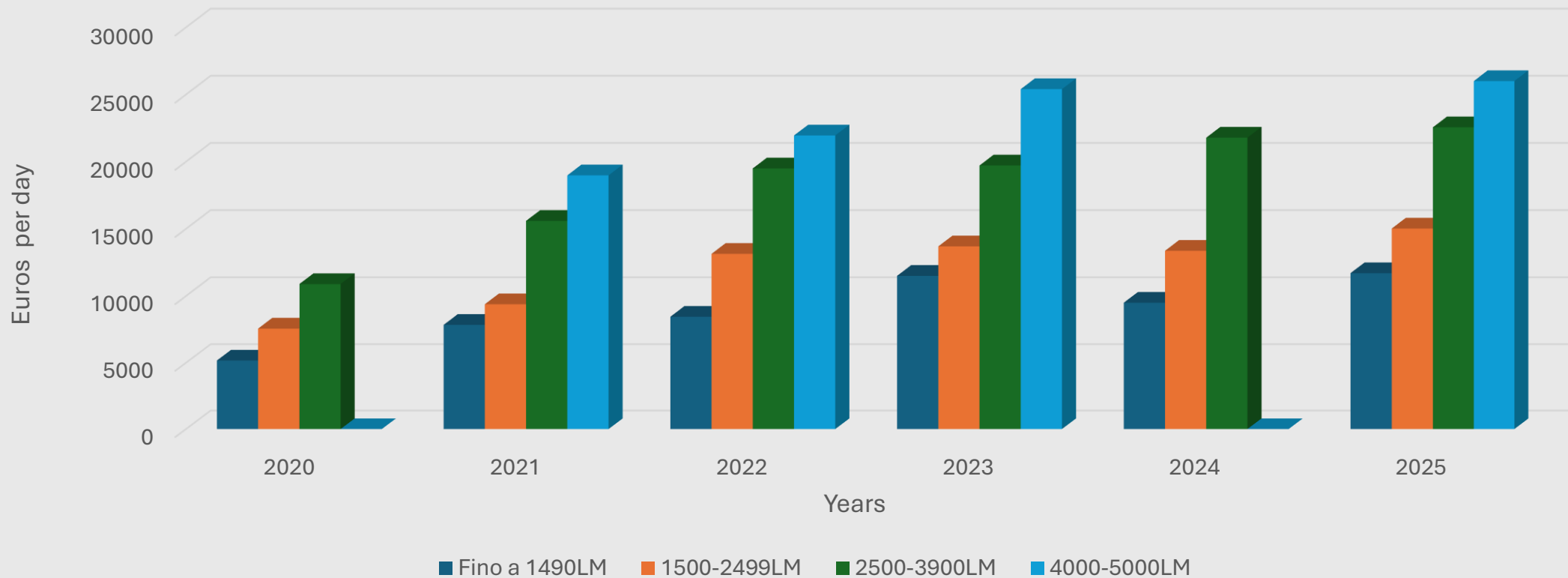
Ro-Ro Market daily time charter hire trend
